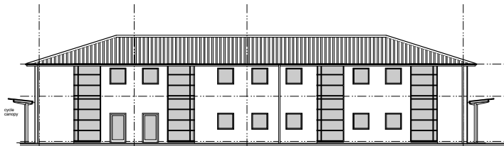
NORTH ELEVATION.
