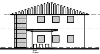
EAST ELEVATION.
